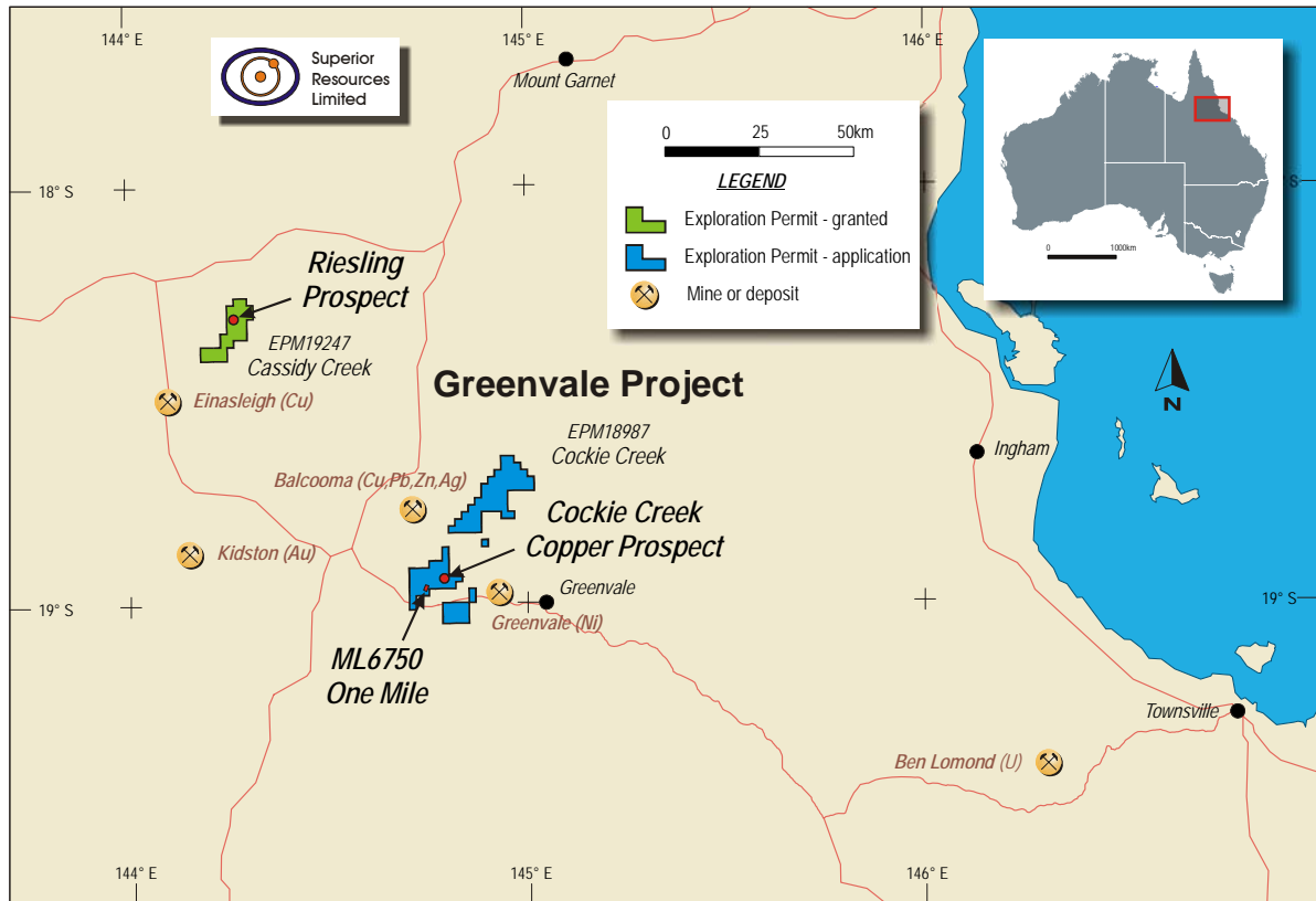
Figure 1. Location of Superior's Greenvale Project and One Mile Mining Lease in northeast Queensland
